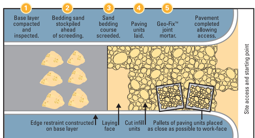
Figure 1 Site layout & paving steps
